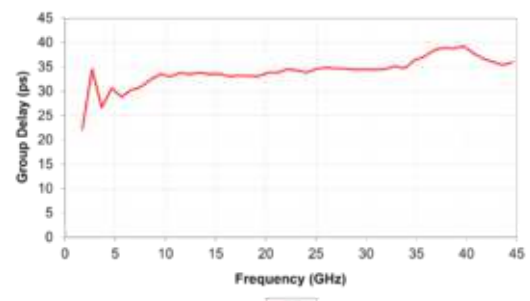
Group Delay
