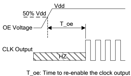
Figure 5. OE Enable Timing (OE Mode Only)
