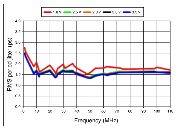
Figure 9. RMS Period Jitter vs Frequency
