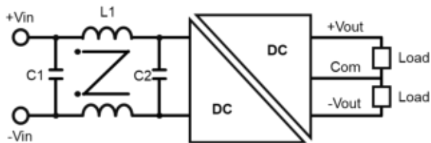
Test set-up
