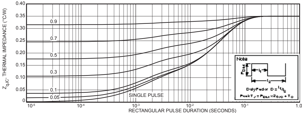
FIGURE 7a, MAXIMUM EFFECTIVE TRANSIENT THERMAL IMPEDANCE, JUNCTION-TO-CASE vs PULSE DURATION
