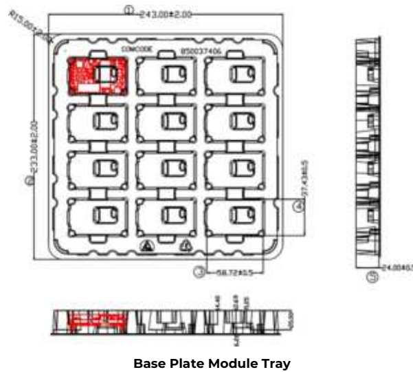
Figure 25. QSDW042 Packaging Tray
