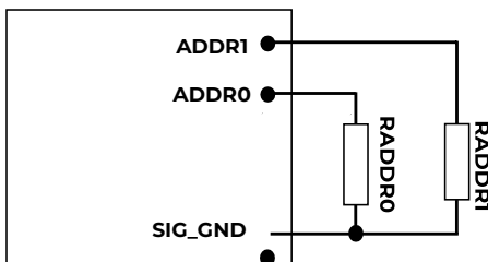
Figure 23. Circuit showing connection of resistors used to set the PMBus address of the module.
