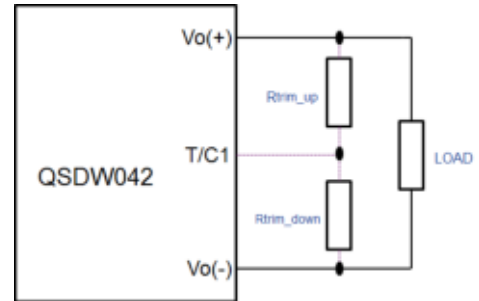
Figure 16. Circuit Configuration to Trim Output Voltage.
