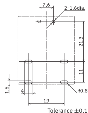
Recommended PC board pattern ( BOTTOM VIEW )
