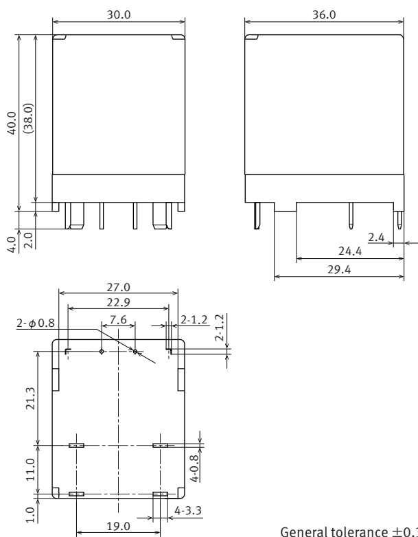
External dimensions
