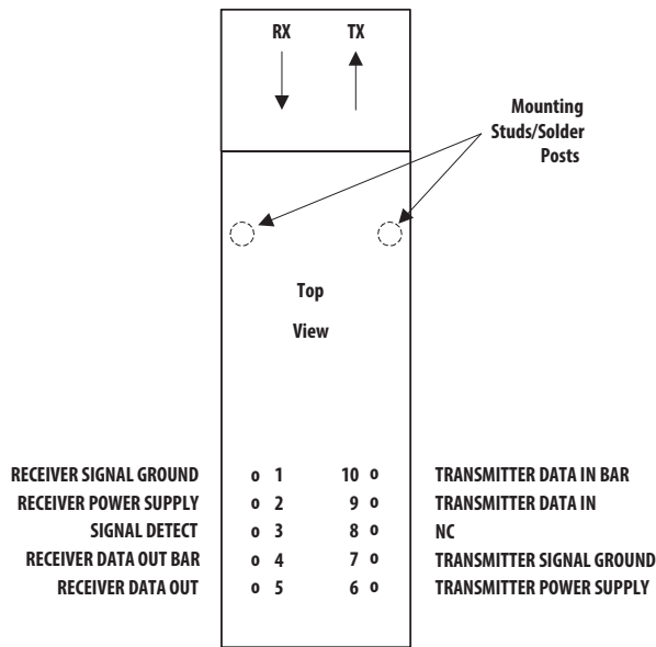
Figure 2: Pinout Diagram
