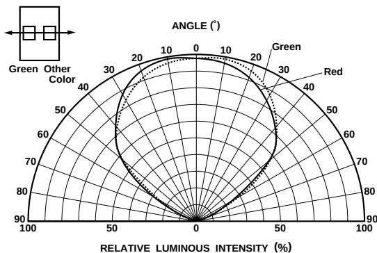
Fig. 1 Directional pattern (1)
