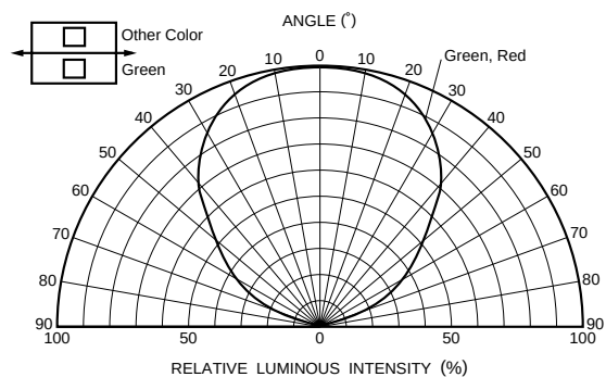
Fig. 2 Directional pattern (2)
