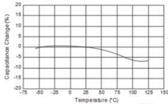
[ Example of Temperature Characteristics X7R(R7) ] Sample: 0.1 \mu F, Rated Voltage 50VDC
