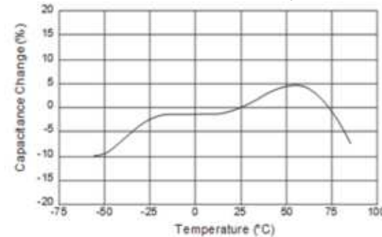
[ Example of Temperature Characteristics X5R(R6) ] Sample: 22 \mu F, Rated Voltage 4VDC
