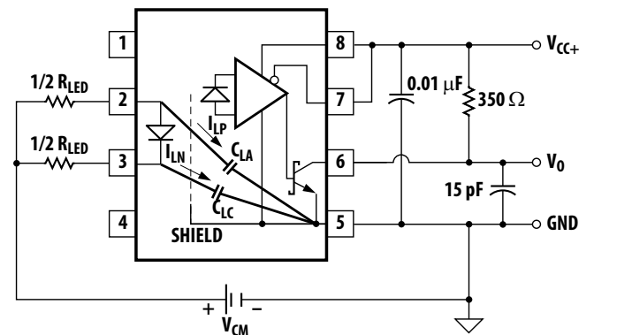
Figure 22: AC Equivalent Circuit
