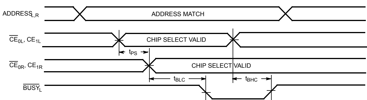
Figure 14. Busy Timing Diagram No. 2 (Address Arbitration) [54]
