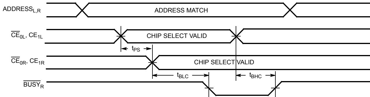
Figure 13. Busy Timing Diagram No. 1 ( \overline{CE} Arbitration) [54]
