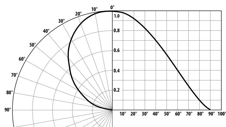
Figure 7: Relative luminous intensity vs. angular displacement for HLMP-08xx
