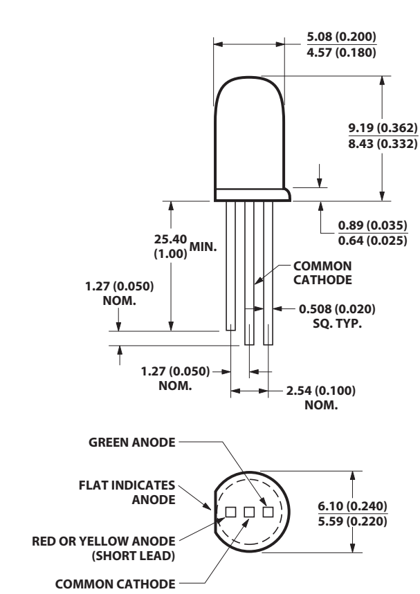
HLMP-40xx Straight Leads
