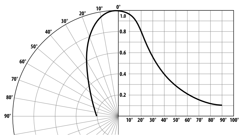
Figure 6: Relative luminous intensity vs. angular displacement for HLMP-40xx
