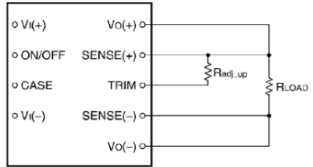
Figure 14. Circuit Configuration to Increase Output Voltage.
