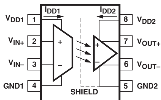
Figure 1: Functional Diagram
