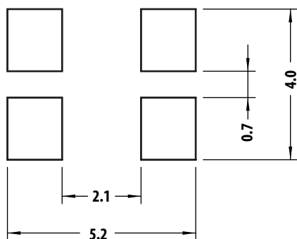
Figure 12 Recommended Soldering Land Pattern
