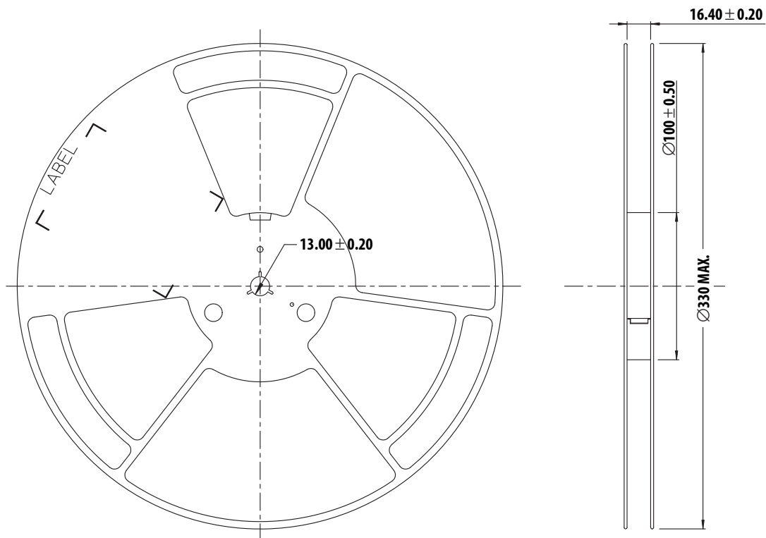
Figure 14 Reel Dimension
