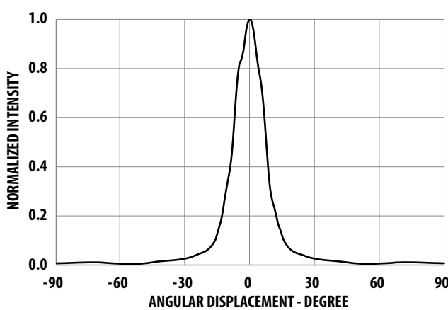
Figure 7 Radiation Pattern for X Axis -15°
