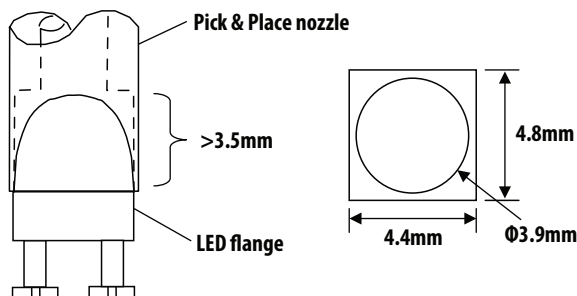
Figure 19 Nozzle Size
