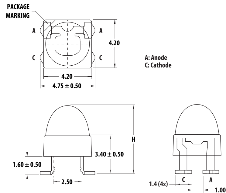
Figure 1 Package Dimensions
