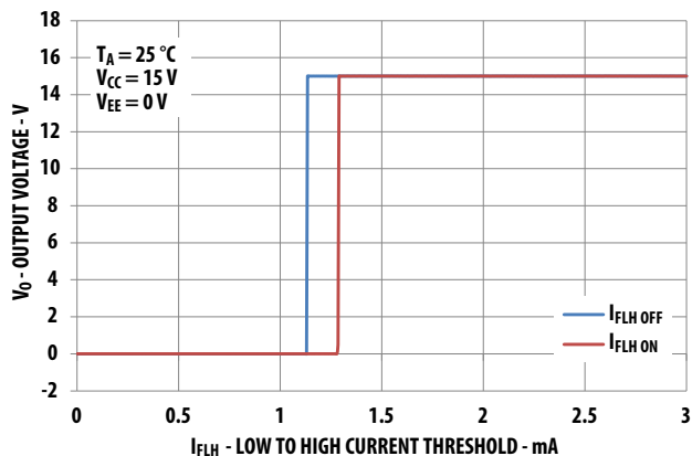
Figure 5: I_{FLH} Hysteresis
