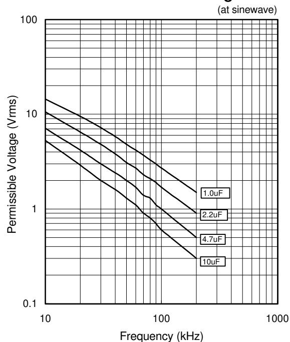
Permissible Voltage
