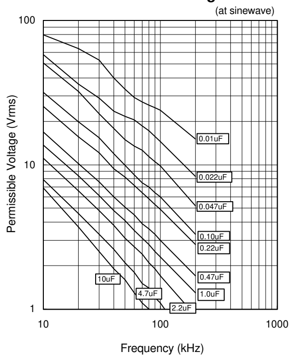
Permissible Voltage
