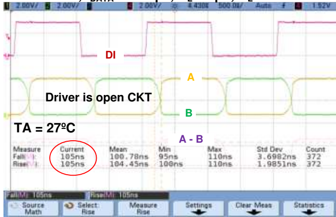
TX Slew-Rate Controlled Output Characteristics: VDD = 3.3V, f DATA = 1Mbps, C L < 1pF, R L = ∞
