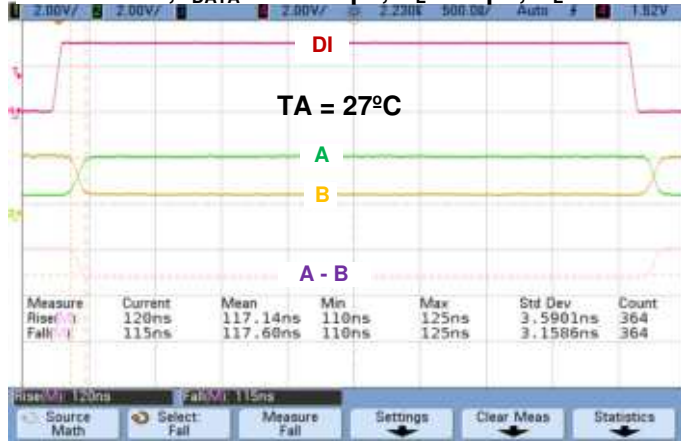
TX Low Speed Output Characteristics: VDD = 3.3V, f DATA = 115Kbps, C L = 50pF, R L = 54Ω
