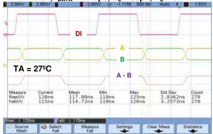
TX Slew-Rate Controlled Output Characteristics: VDD = 3.3V, f DATA = 1Mbps, C L = 50pF, R L = 54Ω
