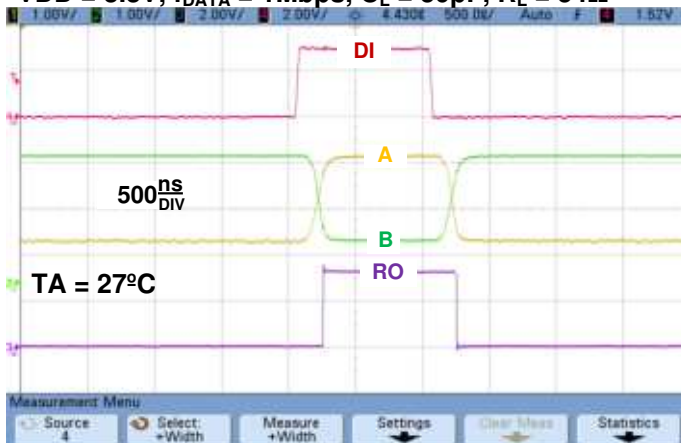
TX / RX Propagation Delay: VDD = 3.3V, f DATA = 1Mbps, C L = 50pF, R L = 54Ω
