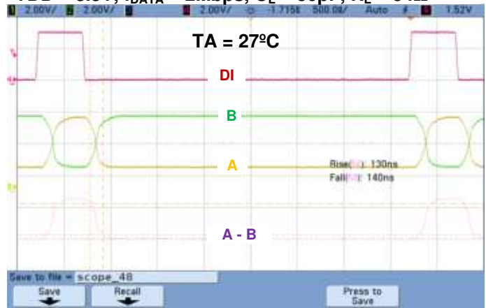
TX High Speed Output Characteristics: VDD = 3.3V, f DATA = 2Mbps, C L = 50pF, R L = 54Ω
