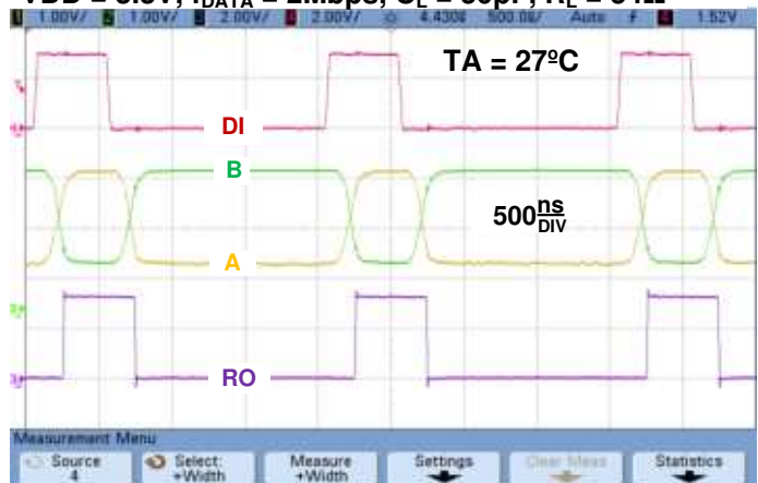
TX / RX Propagation Delay: VDD = 3.3V, f DATA = 2Mbps, C L = 50pF, R L = 54Ω
