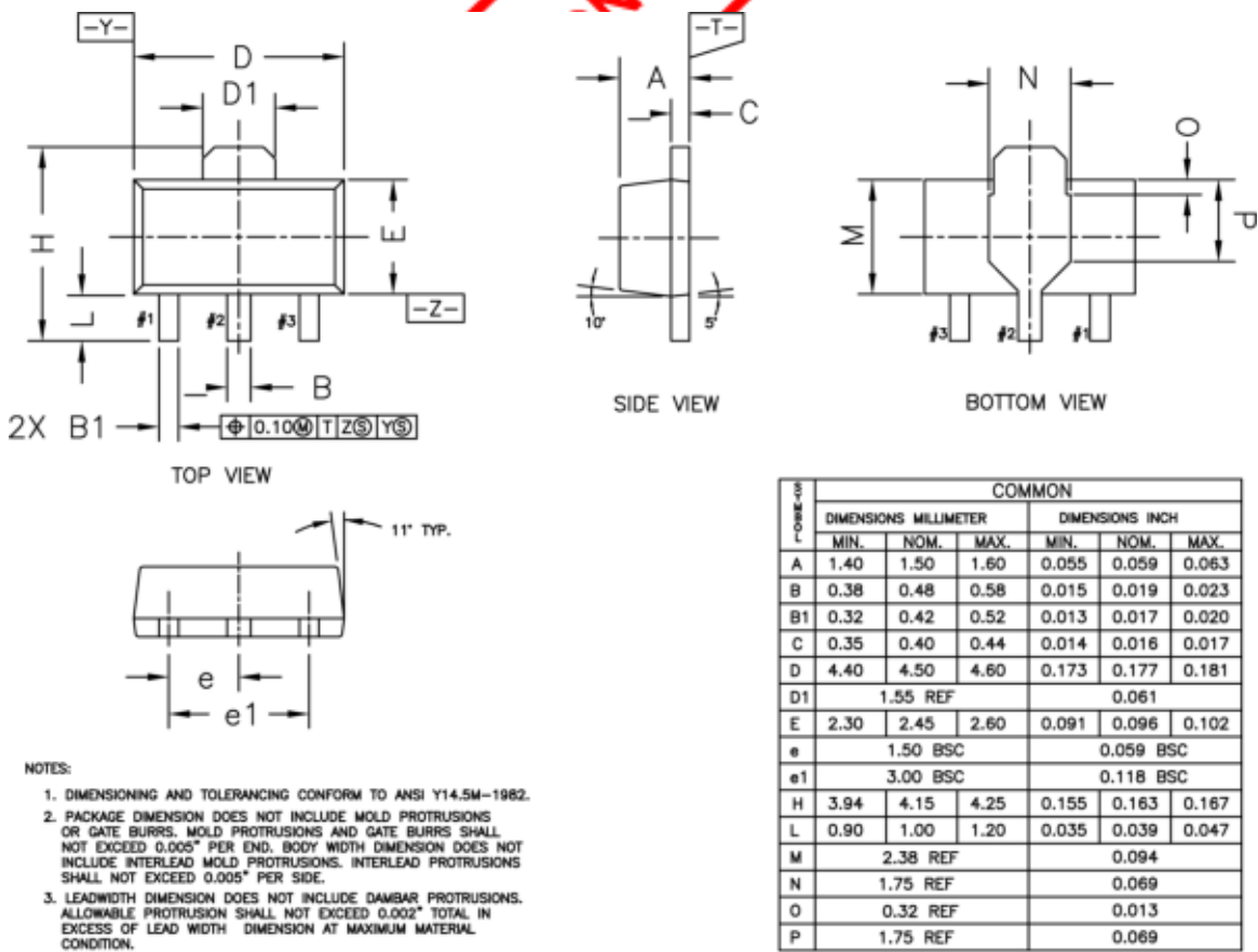
Figure 11. SKY65013-70LF Package Dimensions
