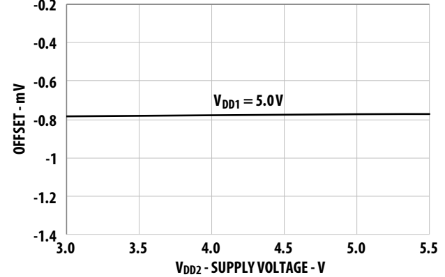
Figure 4: Input Offset vs. Supply V_{DD2}
