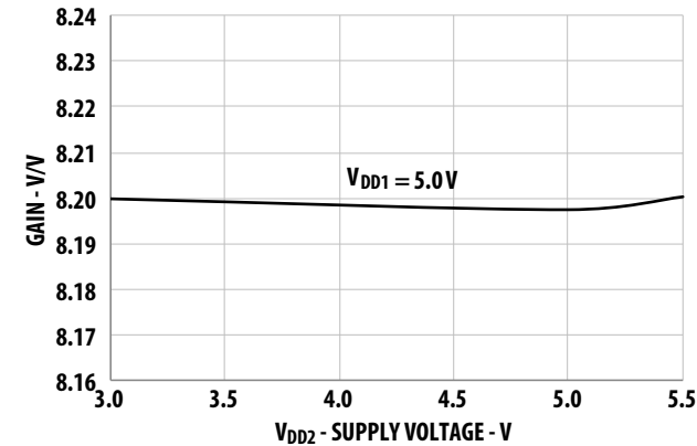
Figure 7: Gain vs. Supply V_{DD2}
