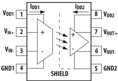
Figure 1: Functional Diagram
