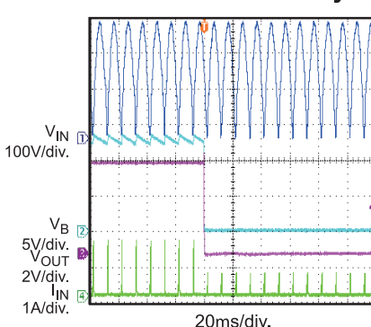
VB Short to GND Protection Entry
