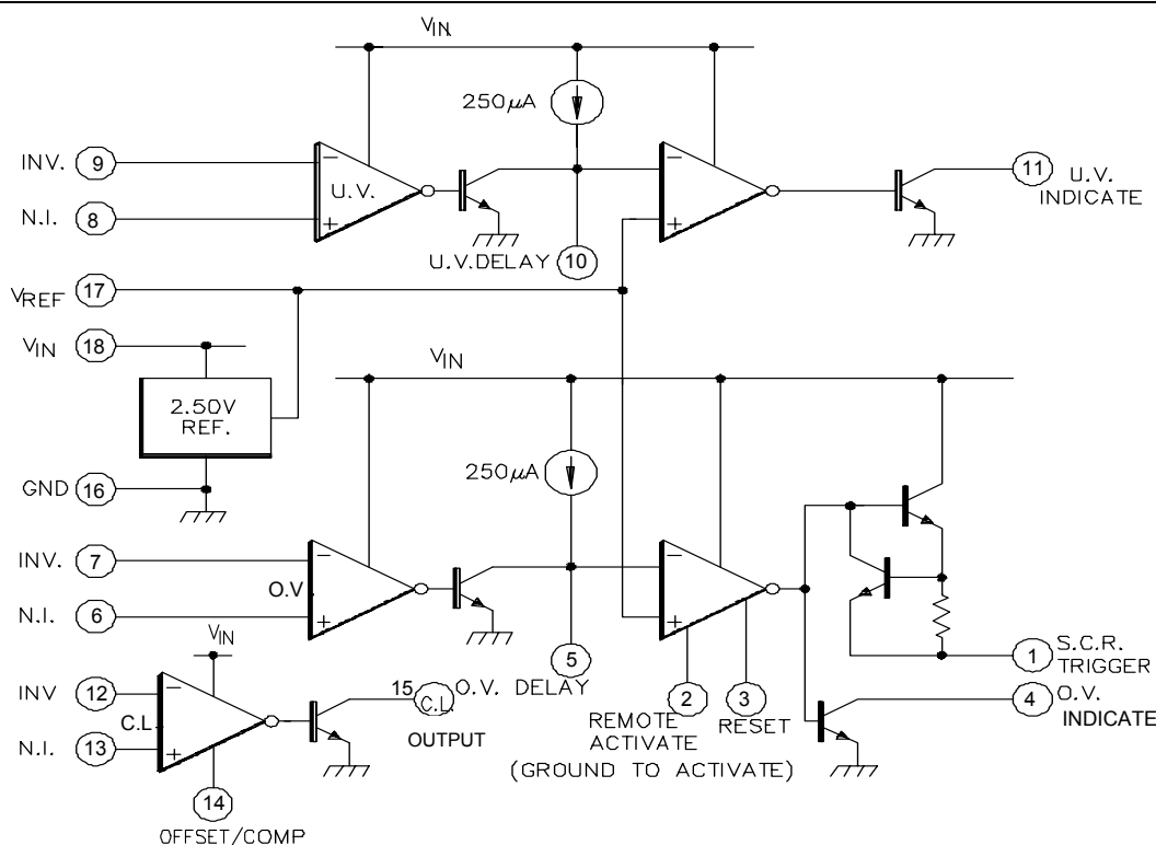
Figure 1 · Block Diagram
