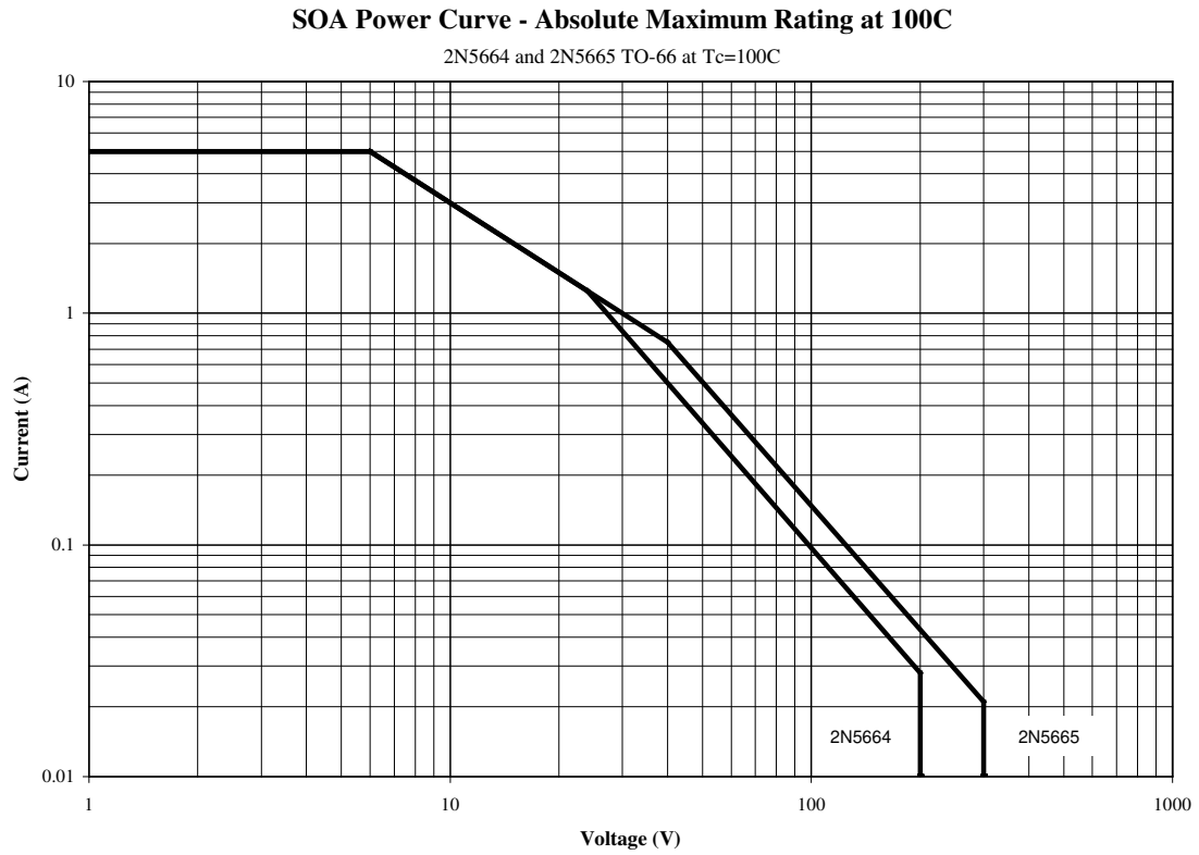
FIGURE 18. Maximum safe operating graph (continuous dc) for types 2N5664 and 2N5665.
