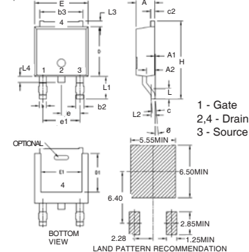
TO-252 AA Outline
