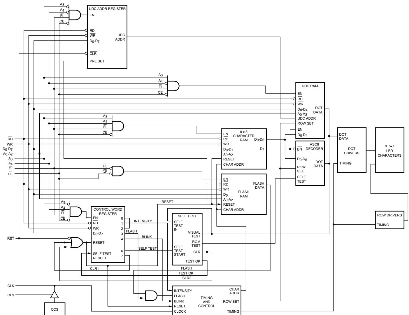
Figure 6: HDSP-210X/-211X/-212X/-250X Internal Block Diagram
