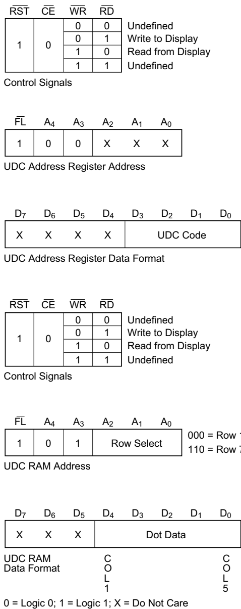
Figure 8: Logic Levels to Access a UDC Character
