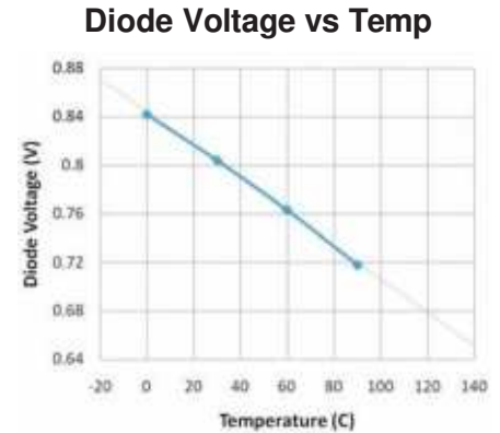
Diode Voltage vs Temp, I_d = 120 \mu A T = (0.84 - V_d) / 0.00133
