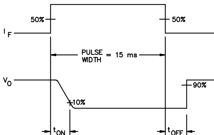
DEVICE TYPES 01,02 AND 04
