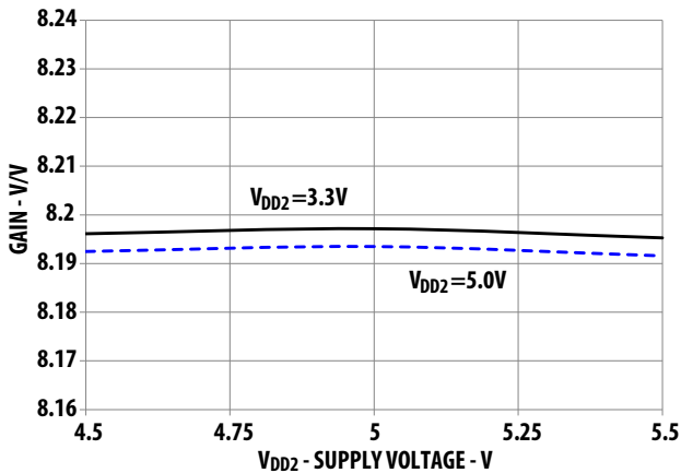
Figure 6: Gain vs. Supply Voltage V_{DD1}
