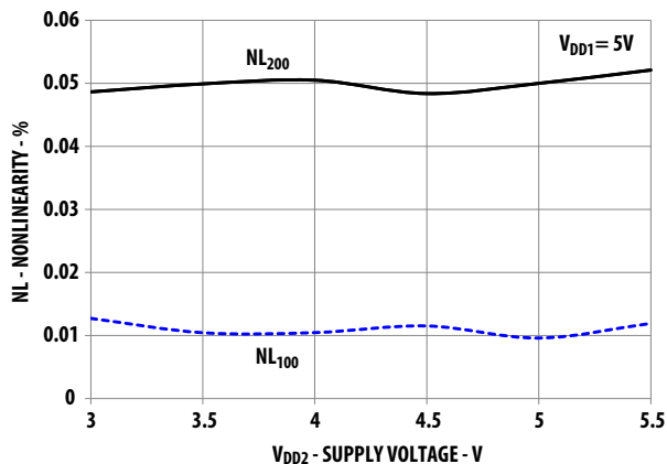
Figure 10: Nonlinearity vs. Supply Voltage V_{DD2}
