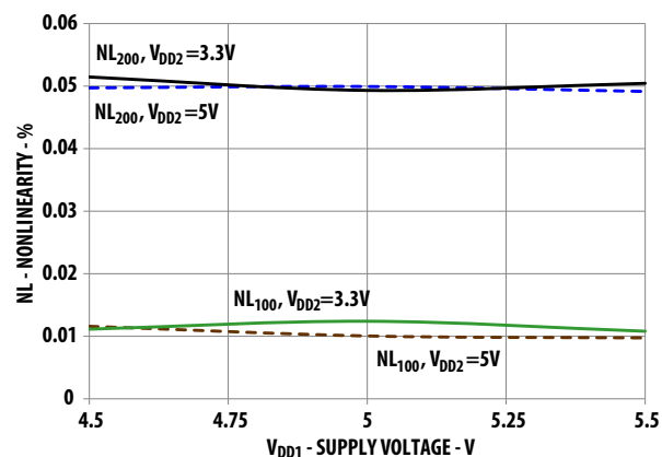
Figure 9: Nonlinearity vs. Supply Voltage V_{DD1}
