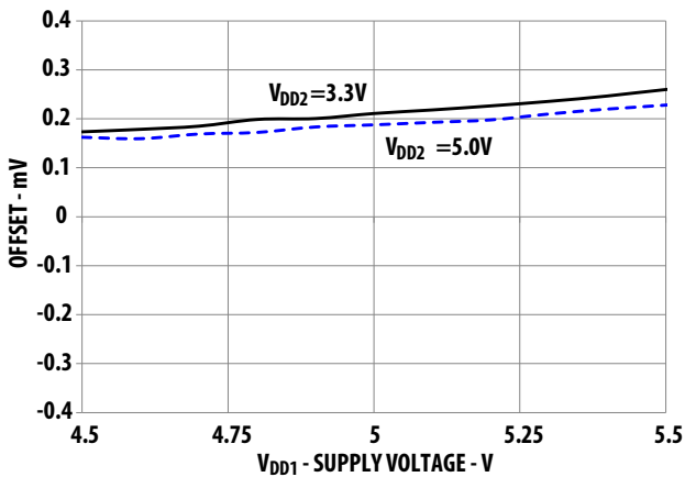
Figure 3: Input Offset vs. Supply Voltage V_{DD1}
