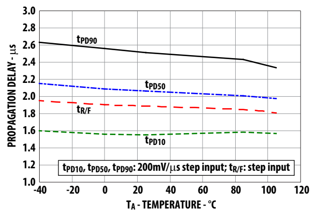
Figure 19: Propagation Delay, Output Rise/Fall Time vs. Temperature
