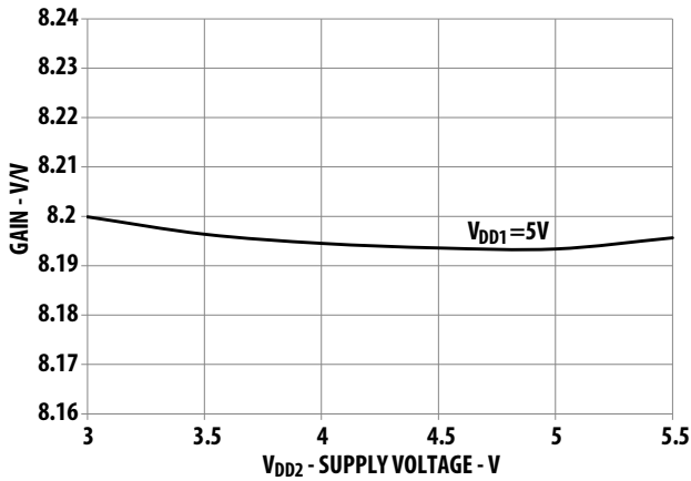
Figure 7: Gain vs. Supply Voltage V_{DD2}
