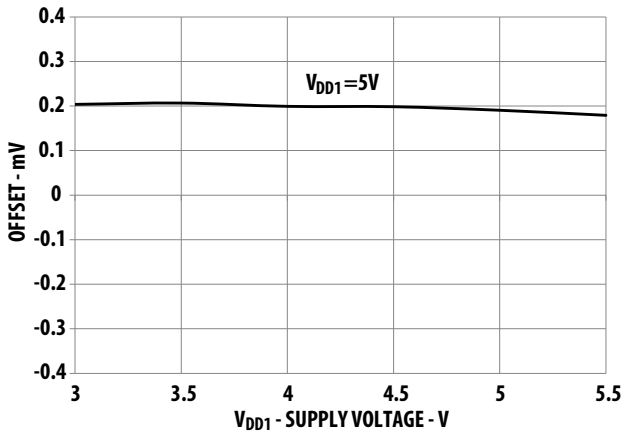
Figure 4: Input Offset vs. Supply Voltage V_{DD2}
