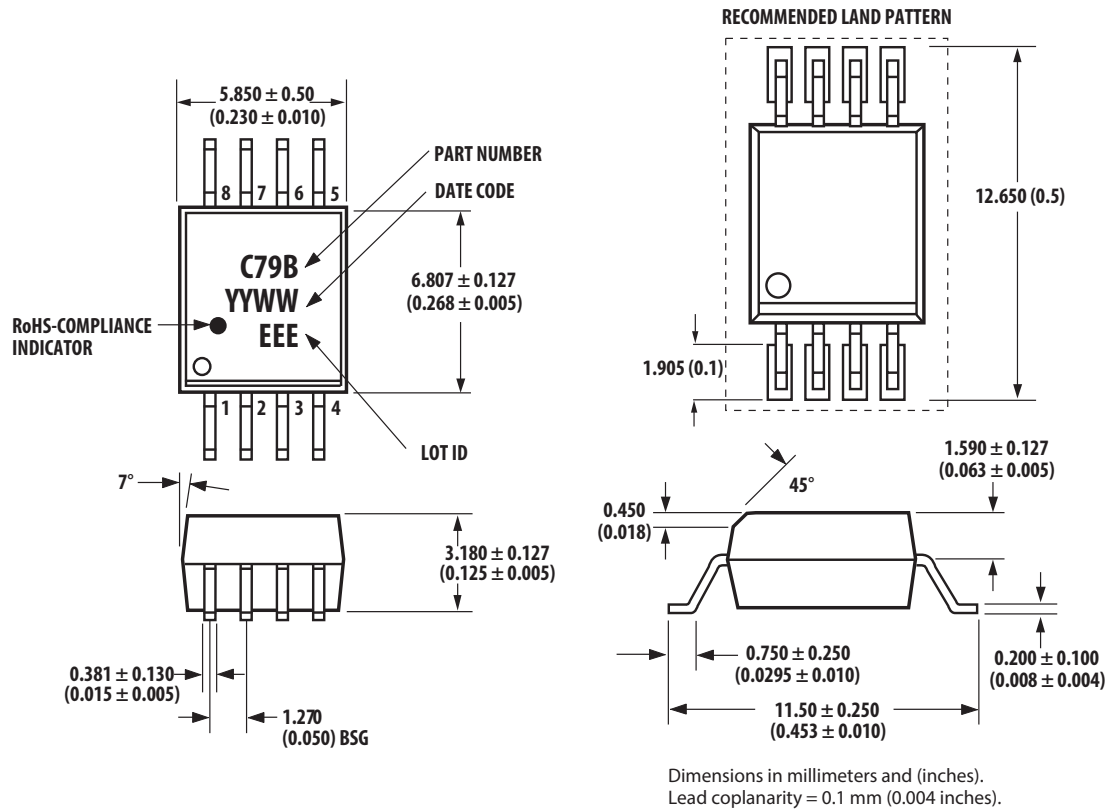
Figure 2: SSO-8 Package
