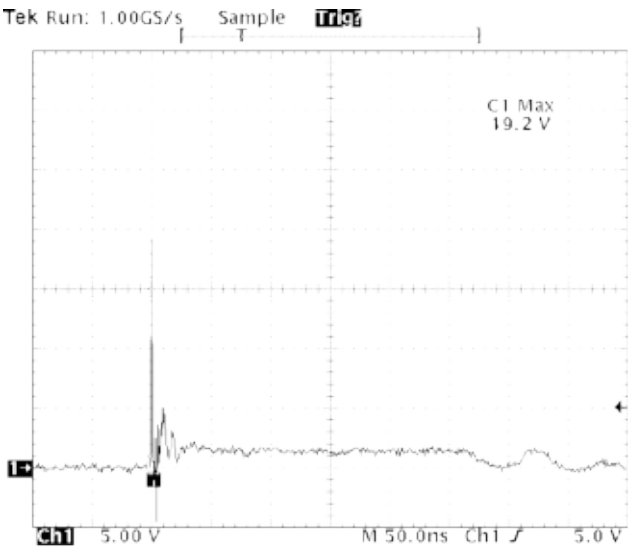
SMF05 ESD Clamping (8kV Contact per IEC 61000-4-2)
