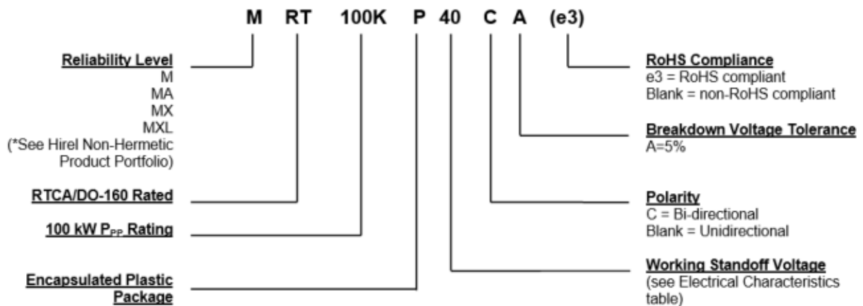
Figure 2-1. Part Nomenclature
