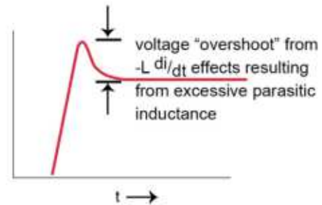
Figure 4-6. Voltage “Overshoot”
