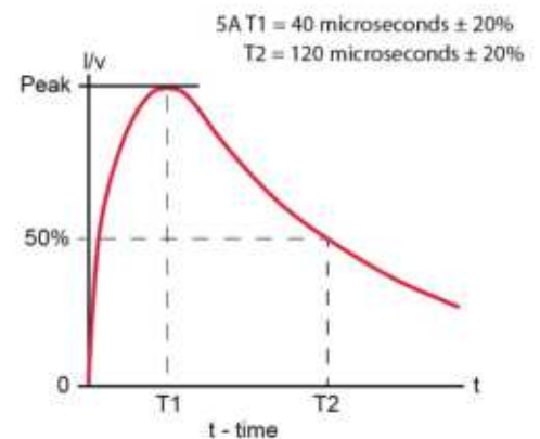
Figure 4-9. Waveform 5A
