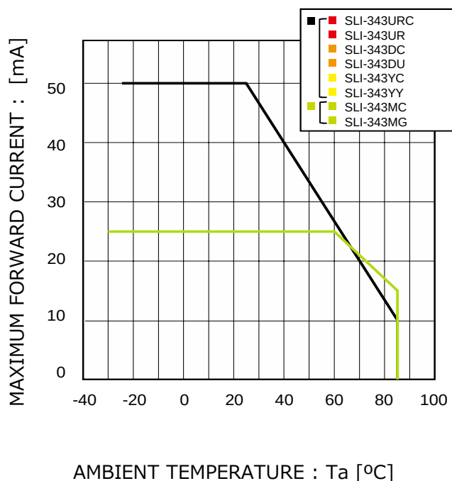
Fig.4 Derating
