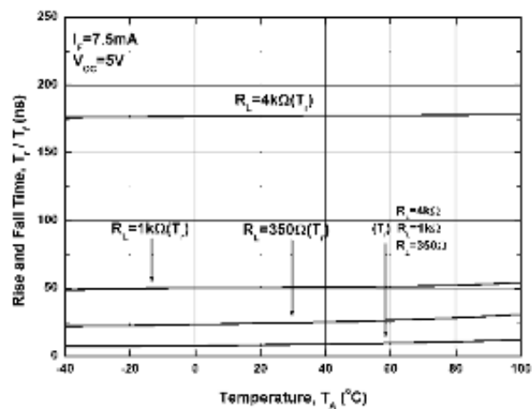
Fig 11 Rise Time / Fall Time vs T_A
