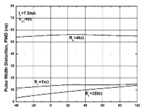
Fig 10 Pulse Width Distortion vs T_A
