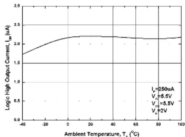
Fig 4 High Level Output Current vs T_A
