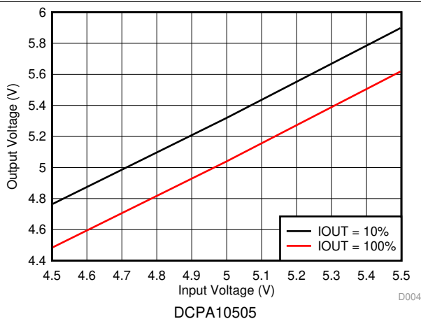
Figure 4. Line Regulation
