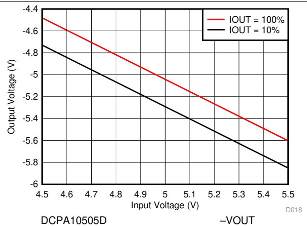
Figure 18. -VOUT Line Regulation
