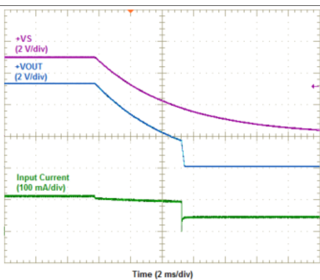
Figure 39. DCPA10505 Turn-OFF
