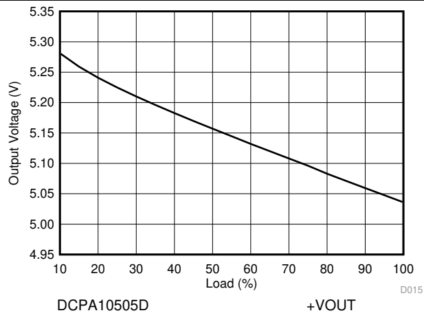
Figure 15. +VOUT Load Regulation
