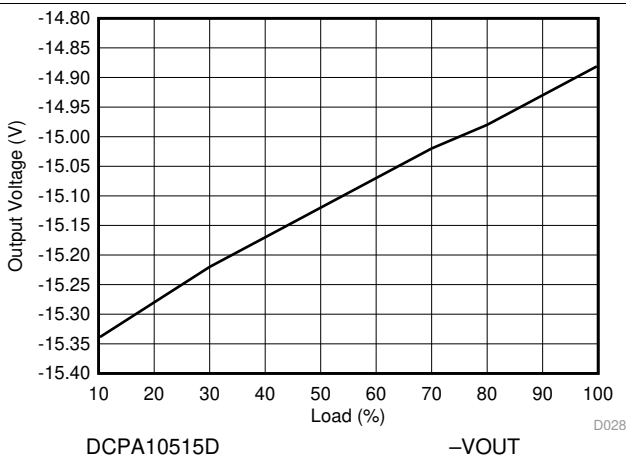
Figure 29. -VOUT Load Regulation
