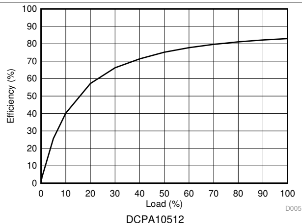
Figure 5. Efficiency versus Load
