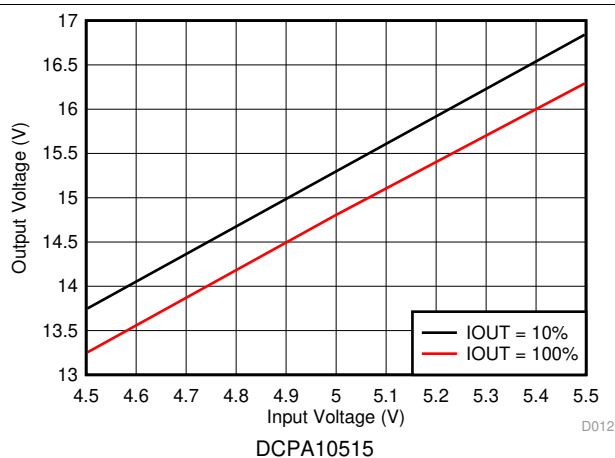
Figure 12. Line Regulation
