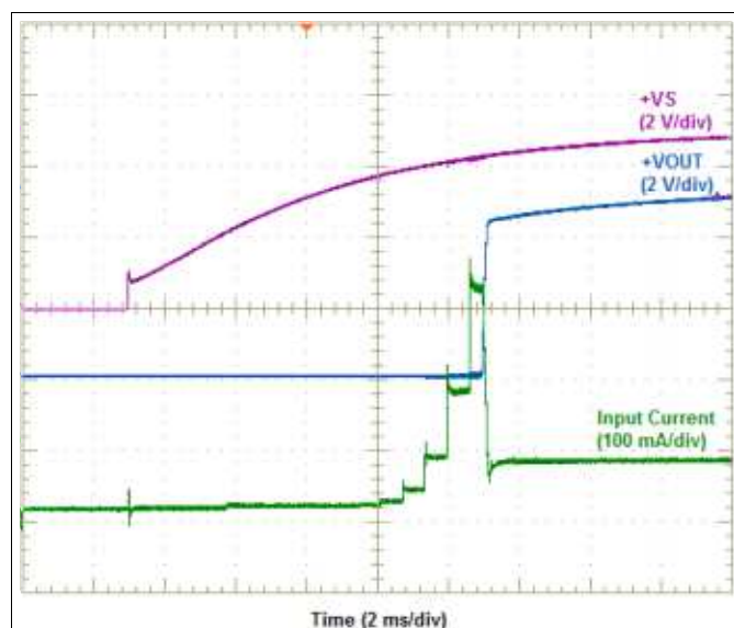
Figure 38. DCPA10505 Turn-ON
