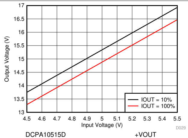
Figure 28. +VOUT Line Regulation
