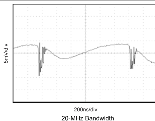
Figure 7-18. DCR010505P Output Voltage Ripple at 100% Load
