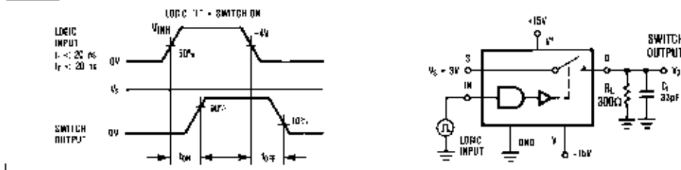
Figure 3. Switching Time Test Circuit
