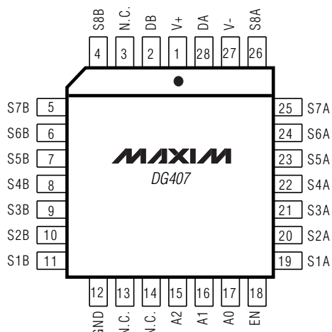
PLCC
