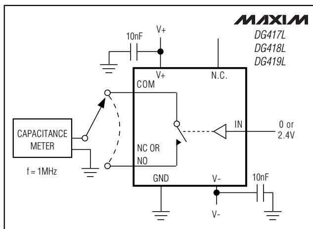
Figure 8. Channel On-Capacitance
