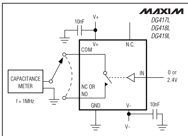
Figure 7. Channel Off-Capacitance
