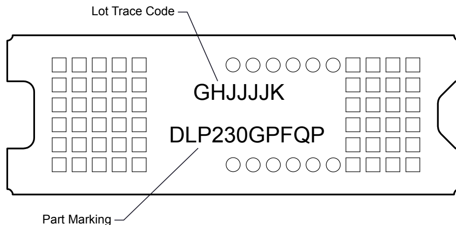
Figure 11-2. DMD Marking
