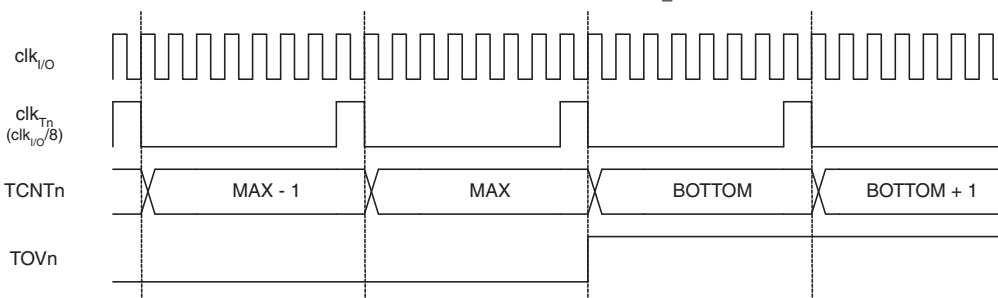
Figure 5. Timer/Counter Timing Diagram, with Prescaler ( f_{\text{clk}_{I/O}}/8 )
