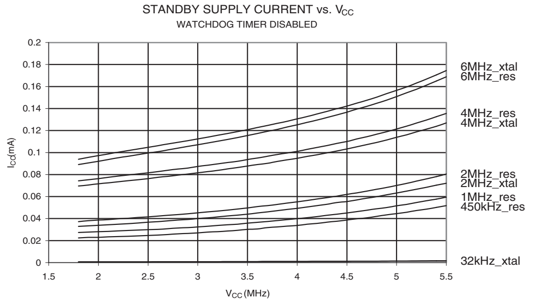
Figure 27-12. Standby Supply Current vs. V_{CC} (Watchdog Timer Disabled)
