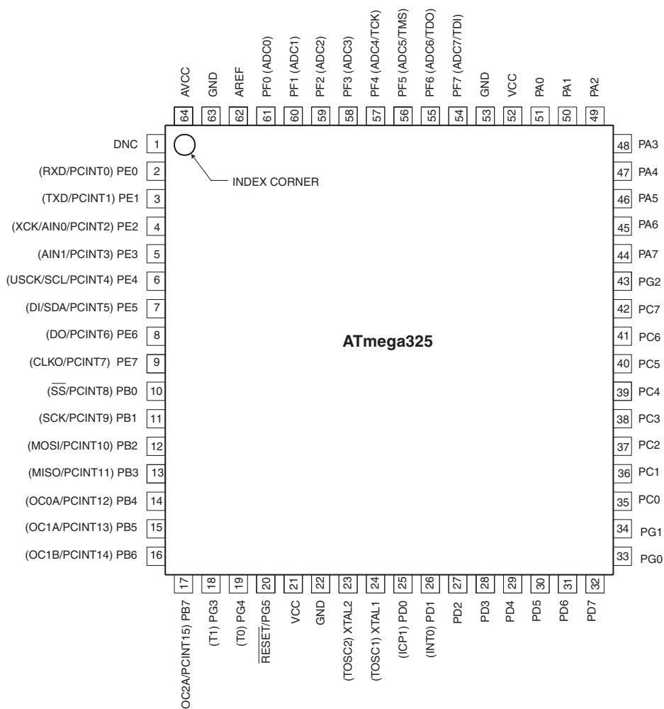
Figure 1-2. Pinout ATmega325P
