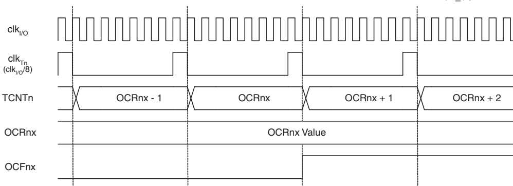
Figure 6. Timer/Counter Timing Diagram, Setting of OCF0A, with Prescaler ( f_{\text{clk}_{I/O}}/8 )
