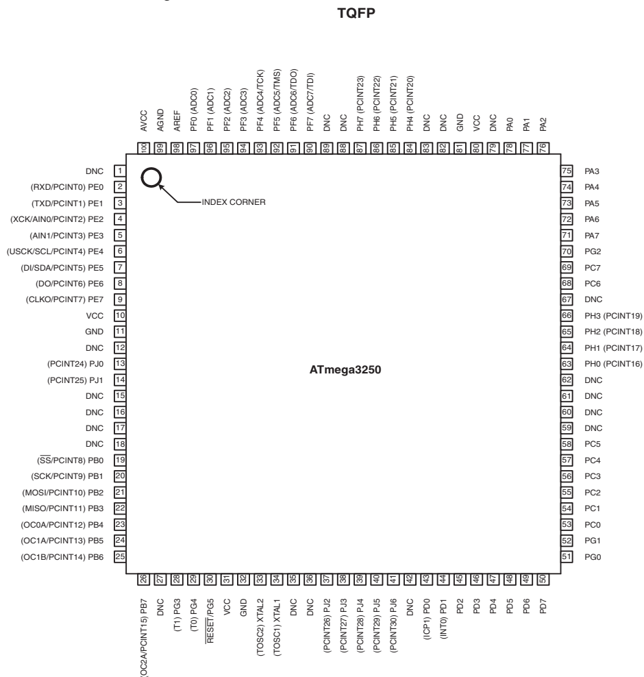
Figure 1-1. Pinout ATmega3250P
