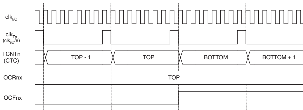
Figure 7. Timer/Counter Timing Diagram, Clear Timer on Compare Match mode, with Prescaler ( f_{\text{clk\_I/O}}/8 )
