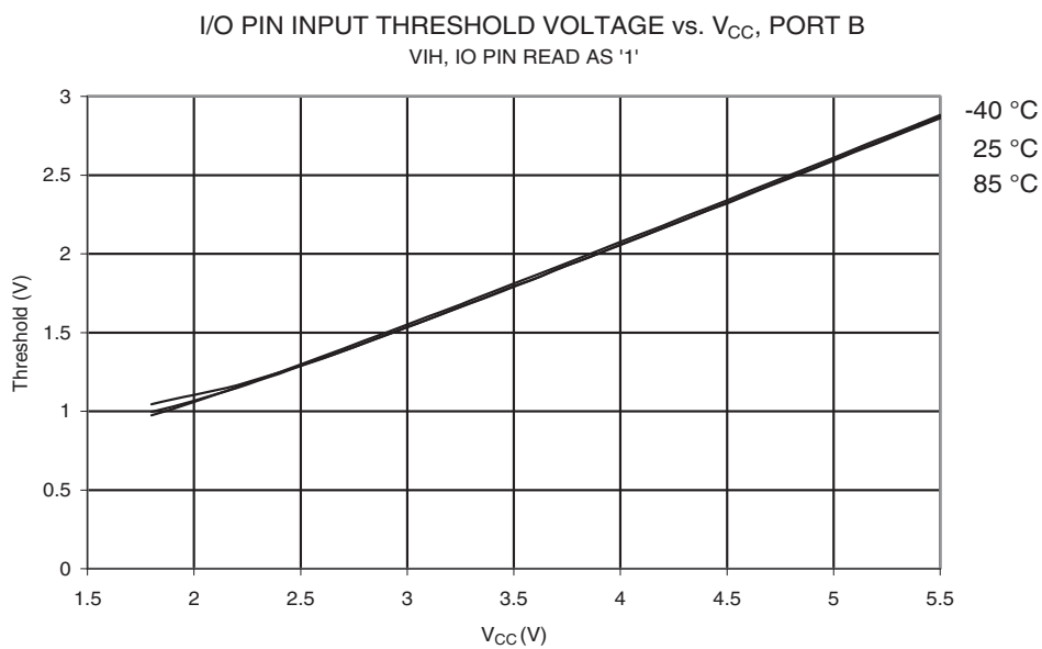
Figure 27-31. I/O Pin Input Threshold Voltage vs. V_{CC} , Port B ( V_{IH} , IO Pin Read as "1")
