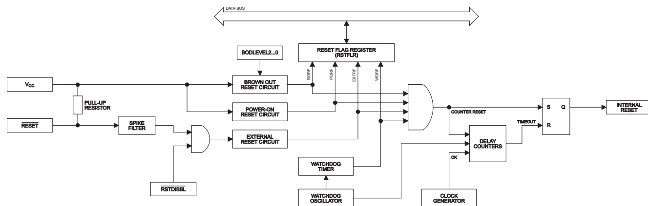
Figure 13. Reset Logic
