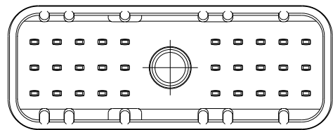
POLARIZATION "B" 581 01 30 002 HOUSING COLOR: BLACK
