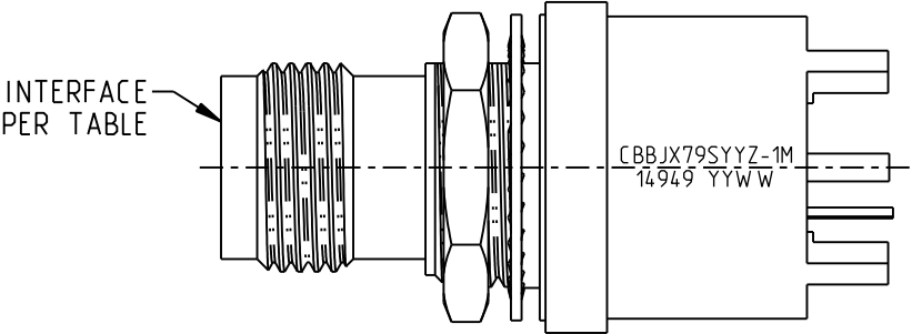
CBBJ379-1M SHOWN
