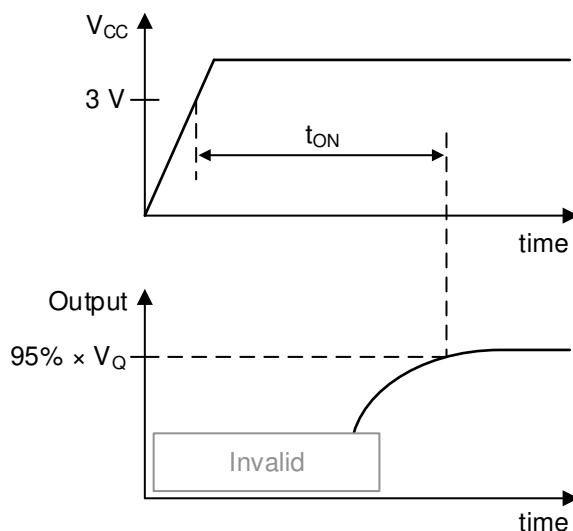
Figure 6-4. t_{ON} Definition
