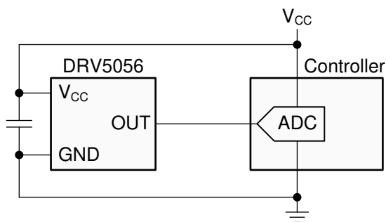
Typical Schematic
