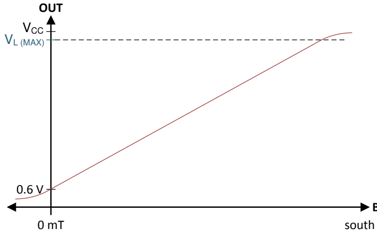
Figure 6-3. Magnetic Response
