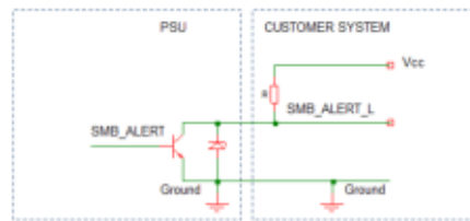
Figure 5. SMB_ALERT_L Connections
