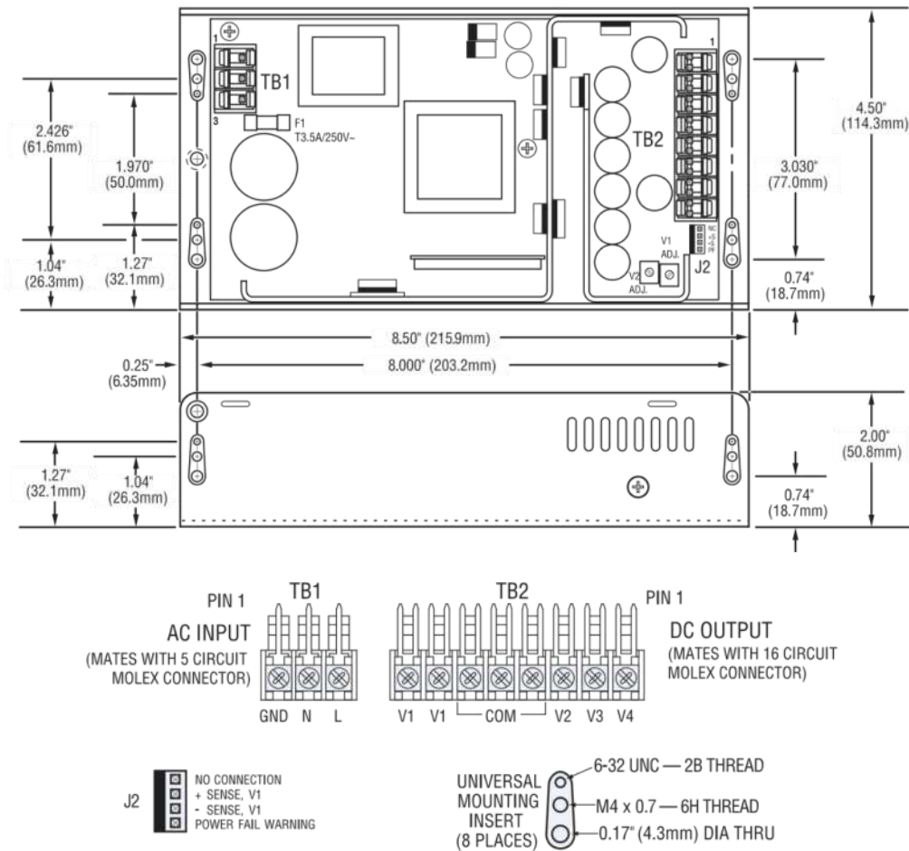
Figure 1. Mechanical Drawing
