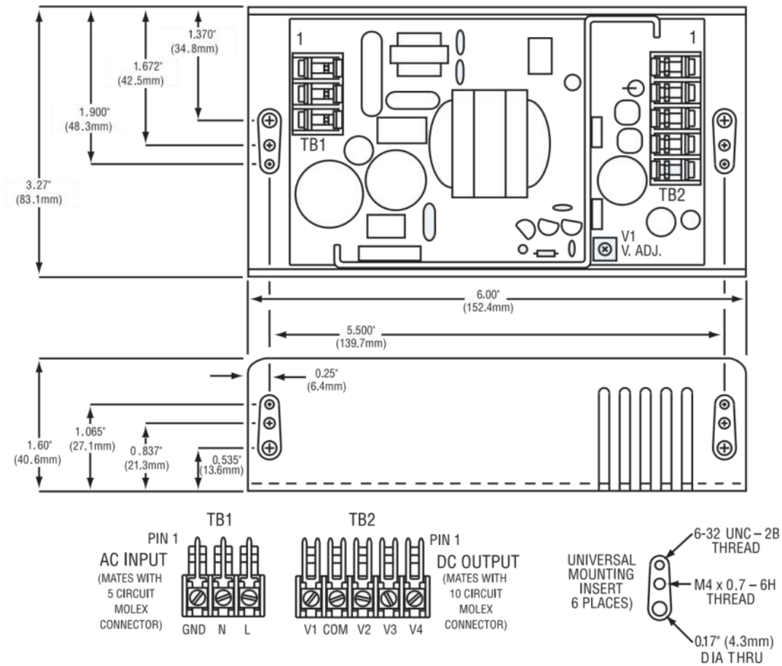
Figure 1. Mechanical Drawing
