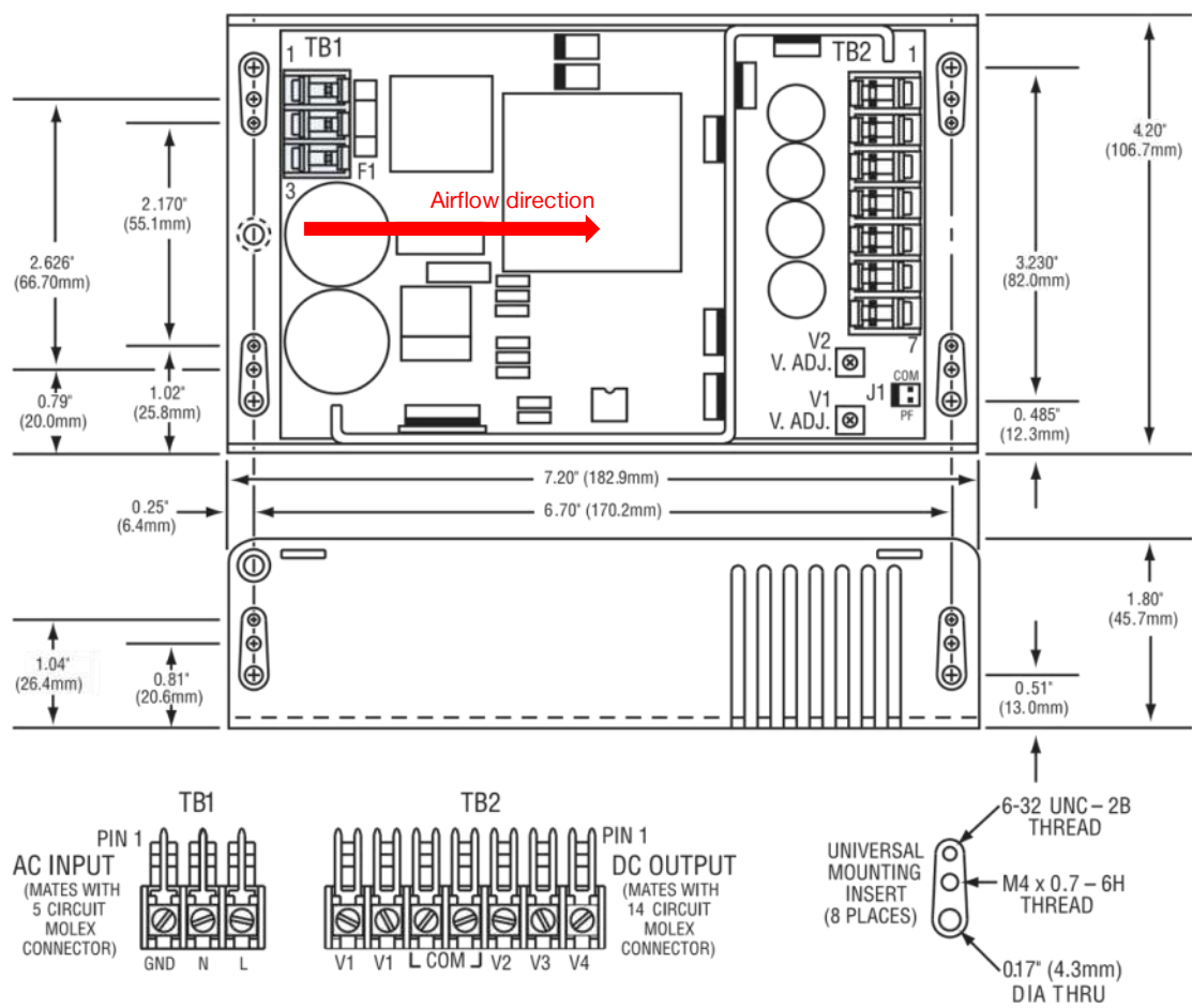
Figure 1. Mechanical Drawing
