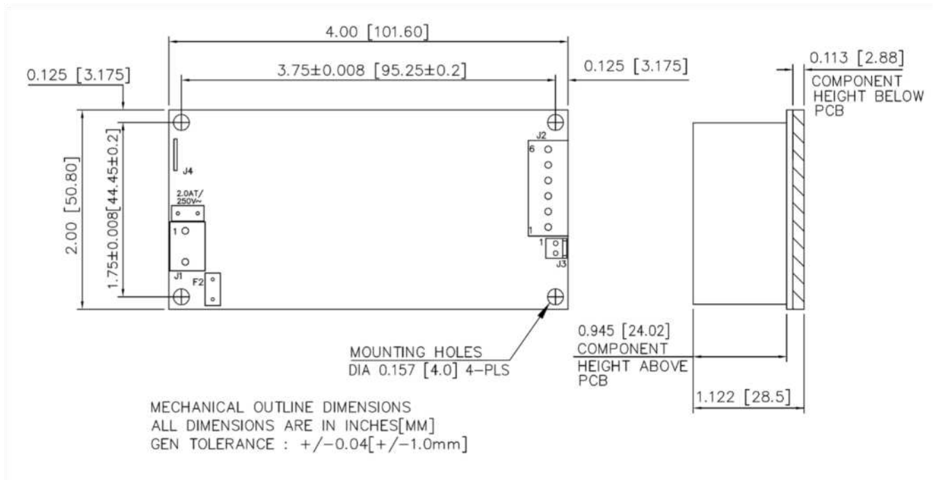
Figure 3. Mechanical Drawing MBC60-1xxxG
