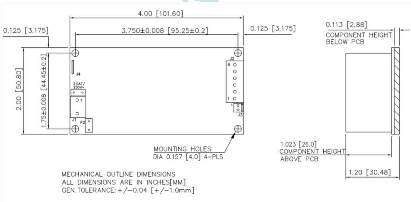
Figure 4. Mechanical Drawing MBC60-3xxxG
