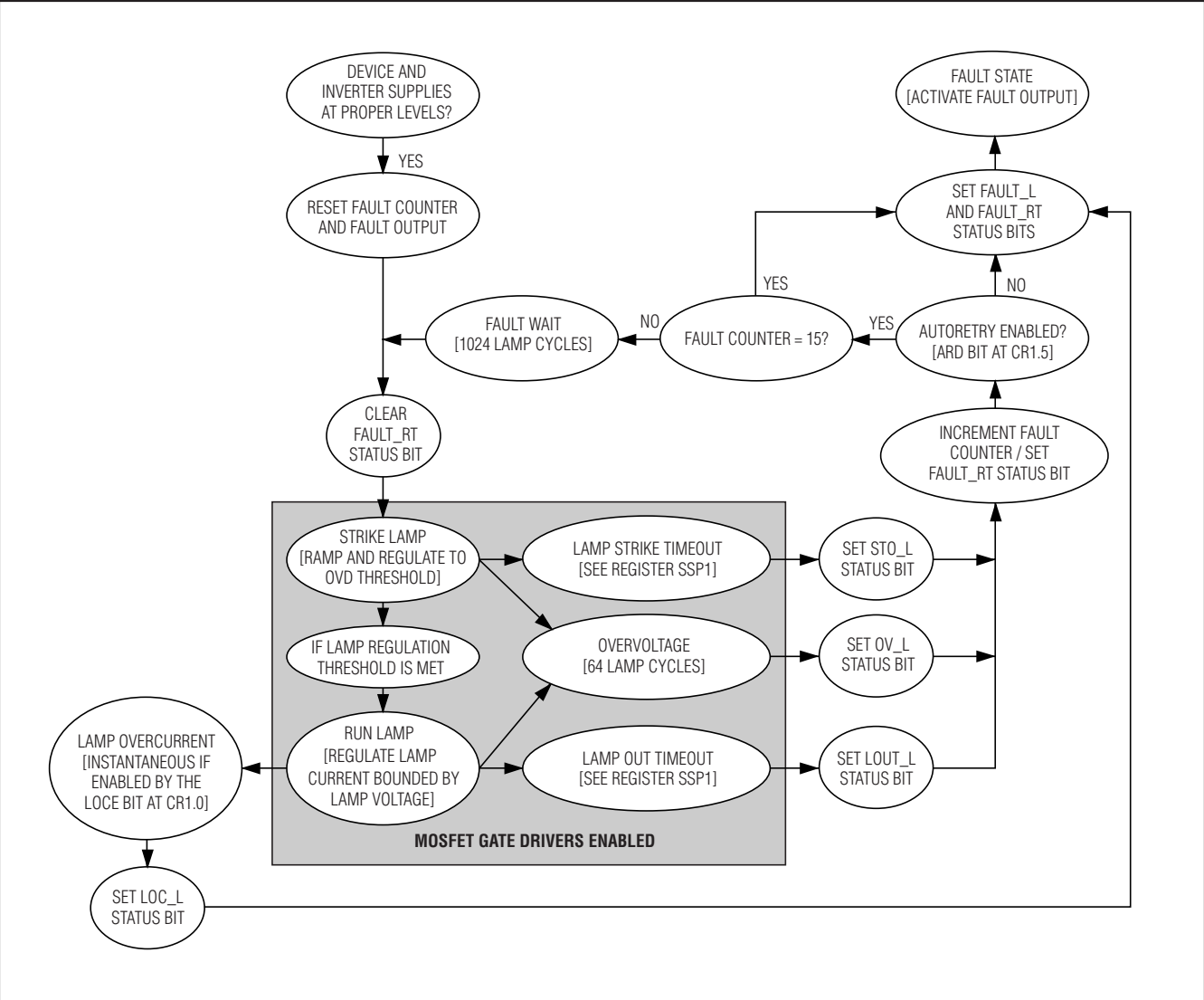
Figure 8. Fault-Handling Flowchart
